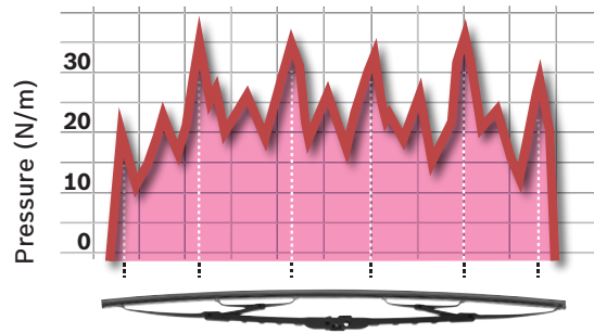
Conventional windshield wiper
